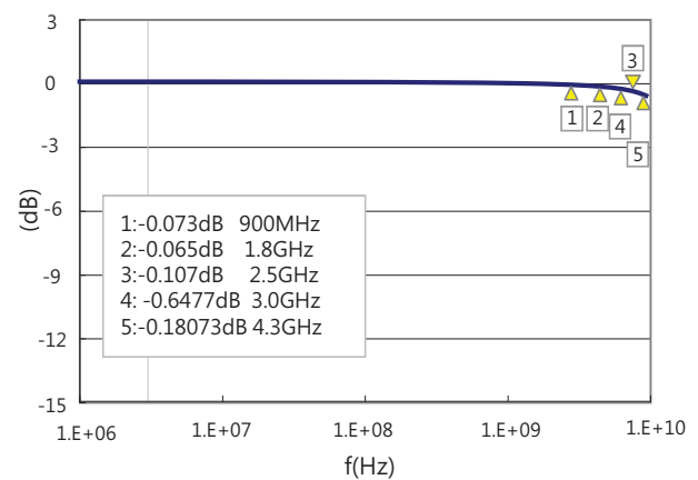
FIG 6 Insertion Loss
