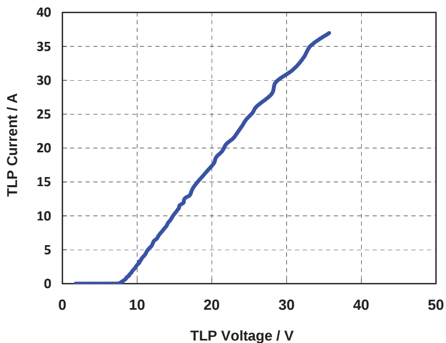
FIG 7 TLP Measurement
