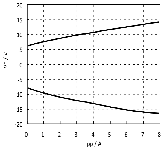
Vc - Ipp ( 25°C )
