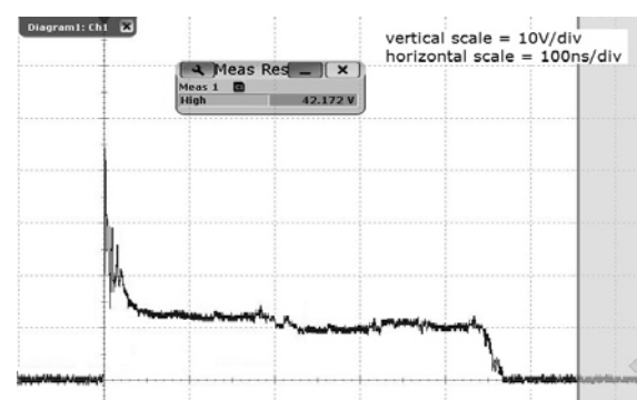
Fig. 8 Clamped +8 kV ESD pulse waveform ( IEC 61000-4-5 network)
