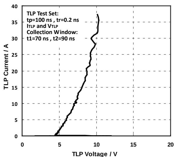
Fig. 9 TLP Measurement
