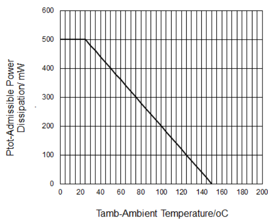
Figure 2. Power De-rating
