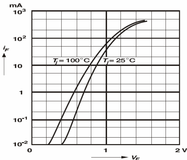
Figure 1. Forward Characteristic
