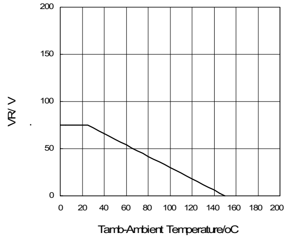
Figure 4. Reverse Voltage De-rating
