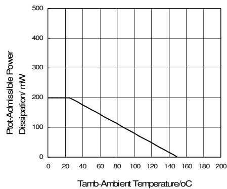
Figure 2. Power De-rating
